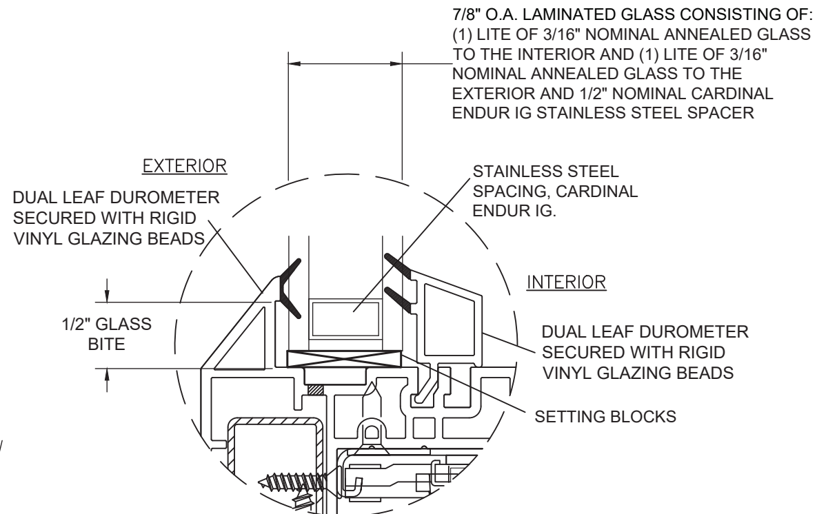
GLAZING DETAIL 1 (SERIES 1310)
