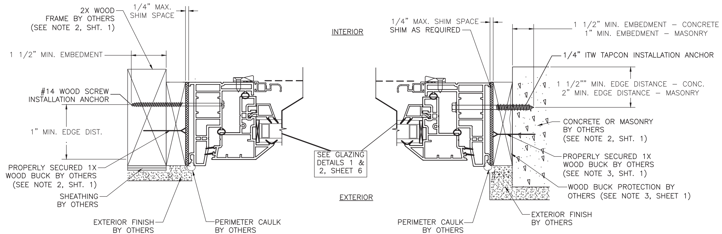
B HORIZONTAL SECTION WOOD FRAME SUBSTRATE
