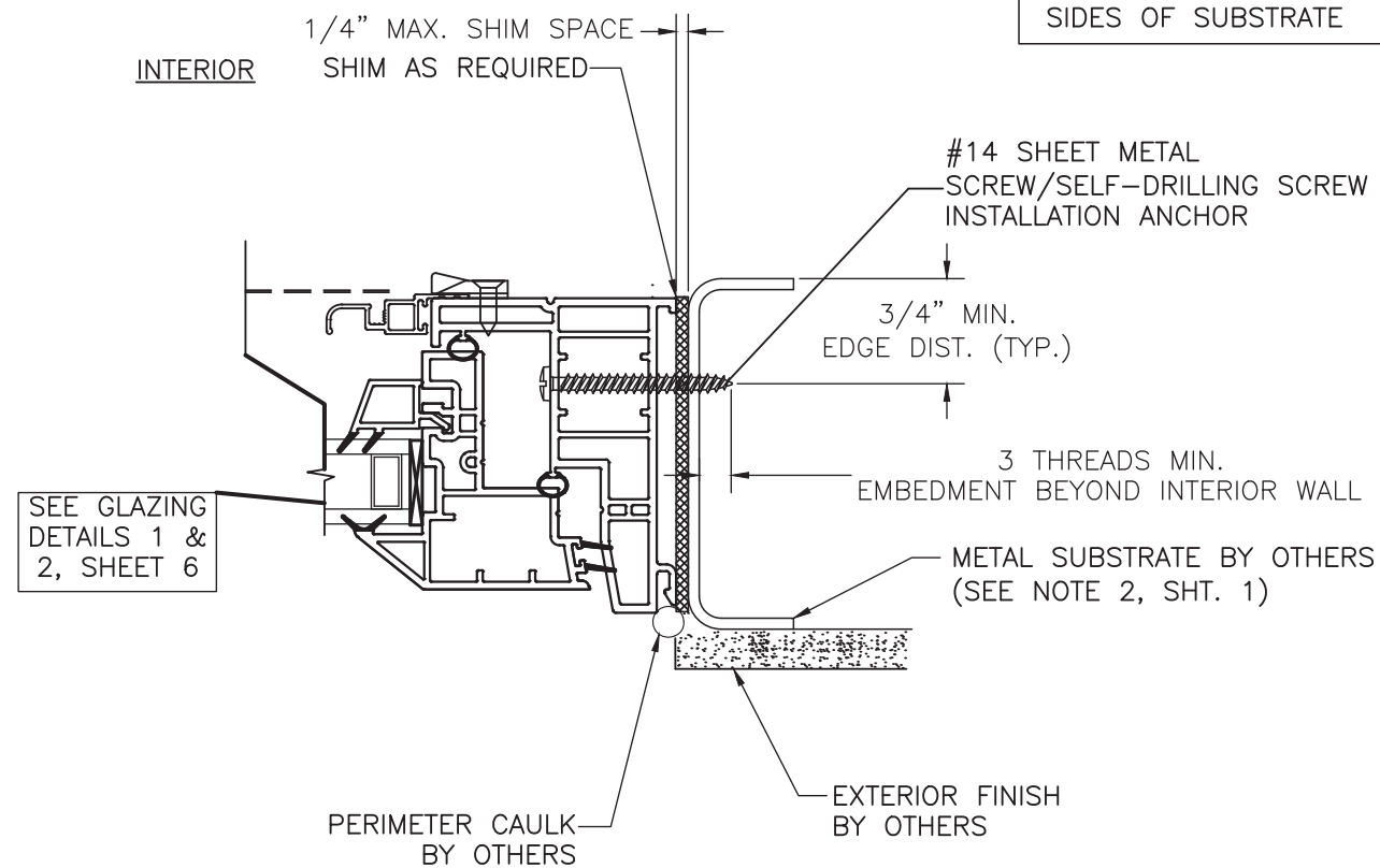
D HORIZONTAL SECTION METAL SUBSTRATE
