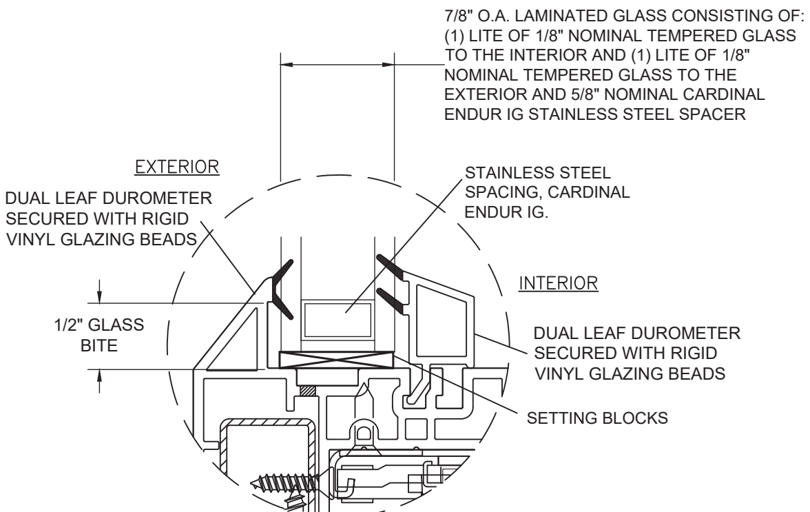
GLAZING DETAIL 2 (SERIES 2010)
